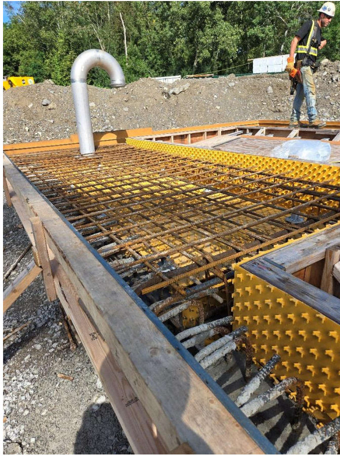
Photo 13: September 2 (pumping station)
