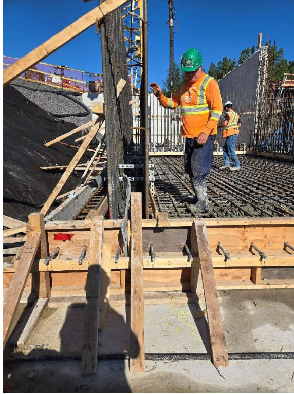
Photo 5: August 18 (tank slab)
