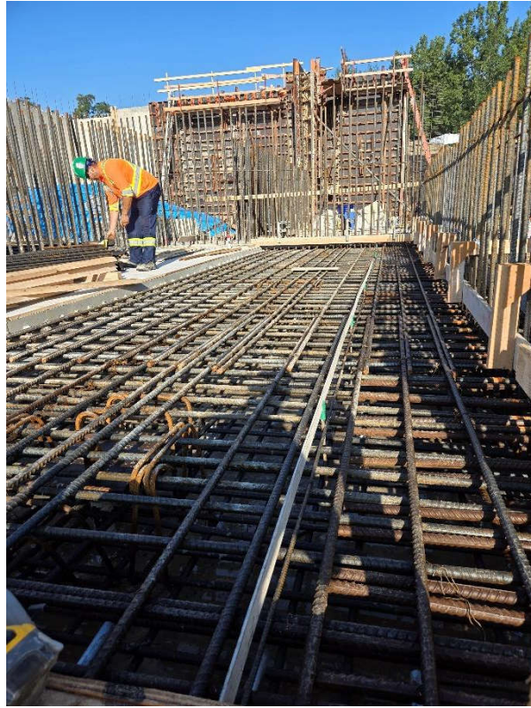
Photo 9: August 26 (tank rebar)
