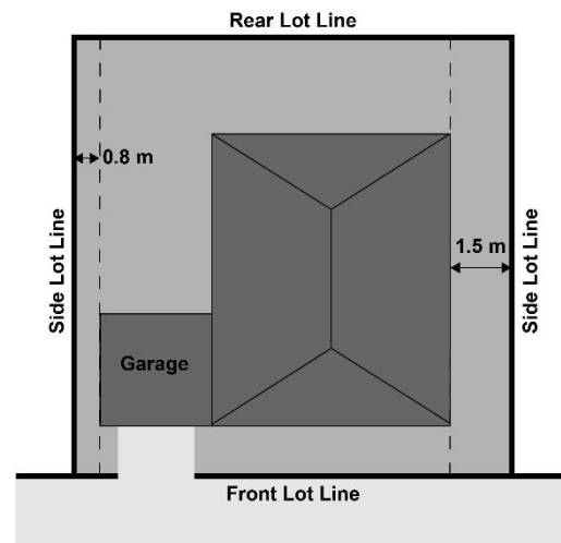
Illustration of Section 4.2 d) Minimum Interior Side Yard Setback Requirements:
