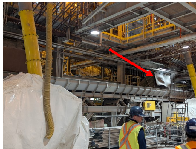
Photo 18: View of operational ash chute cover/baffle.
