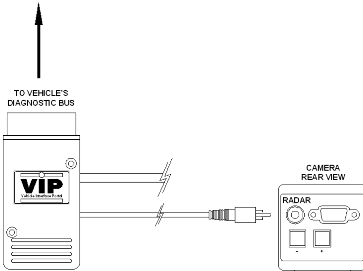
Figure 2.5.3 VIP connection to Video Camera
