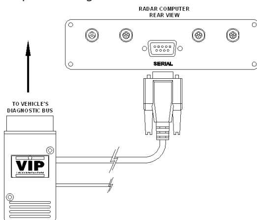
Figure 2.5.1 VIP connection to Radar
