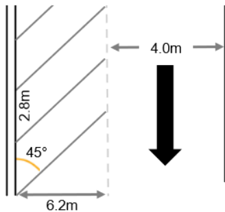
Figure 7.3 – 45-degree parking stalls and drive aisle dimension requirements
