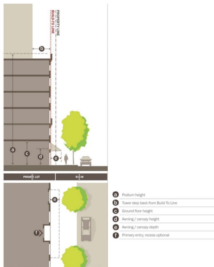
Figure 9.7 Linear Building Frontage on a Podium
