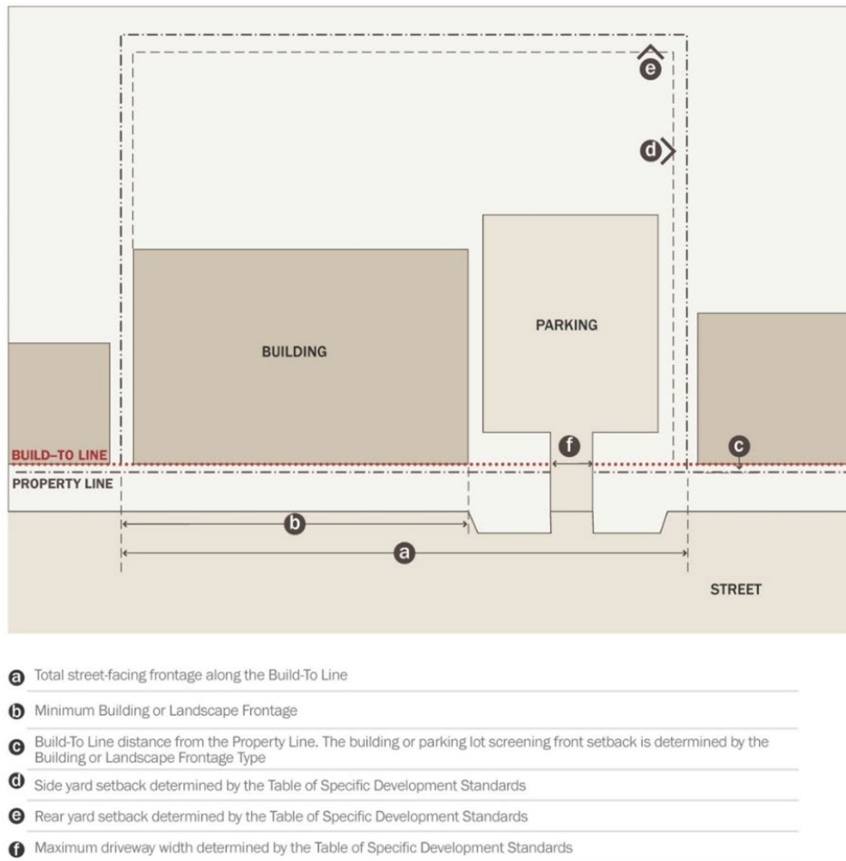
Figure 9.4 Building Siting
