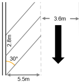
Figure 7.2 – 30-degree parking stalls and drive aisle dimension requirements
