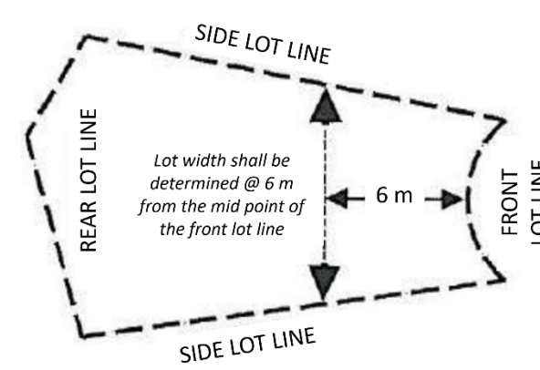
Figure 1.5 – Lot Width Calculation for Pie Lots
