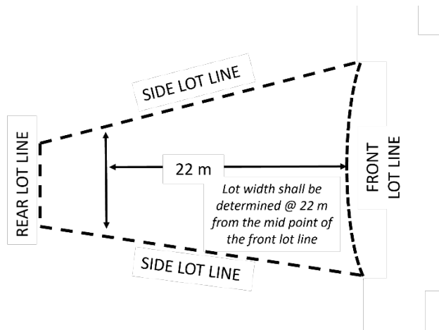
Figure 1.6 – Lot Width Calculation for Reverse Pie Lots
