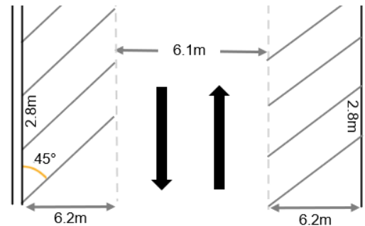
Figure 7.3 – 45-degree parking stalls and drive aisle dimension requirements
