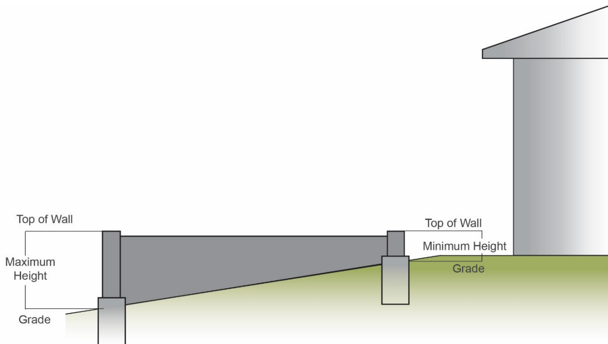
Figure 1.2 Retaining Wall
