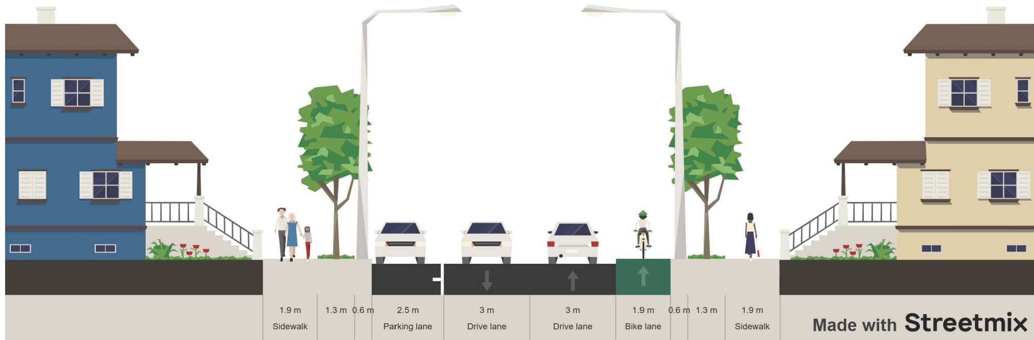
Figure 3: Road redesign example. Diagram is for illustrative purposes only.
